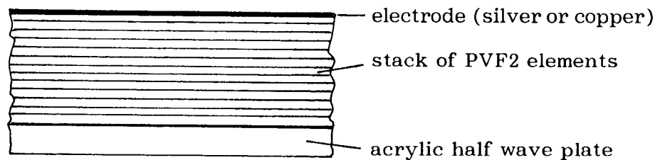
Fig. 2 Composition of bonded element
