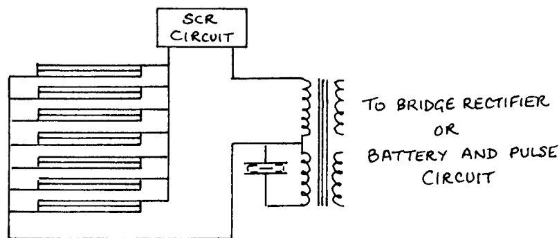
Fig. 6 Series-parallel connections of laminar stack
